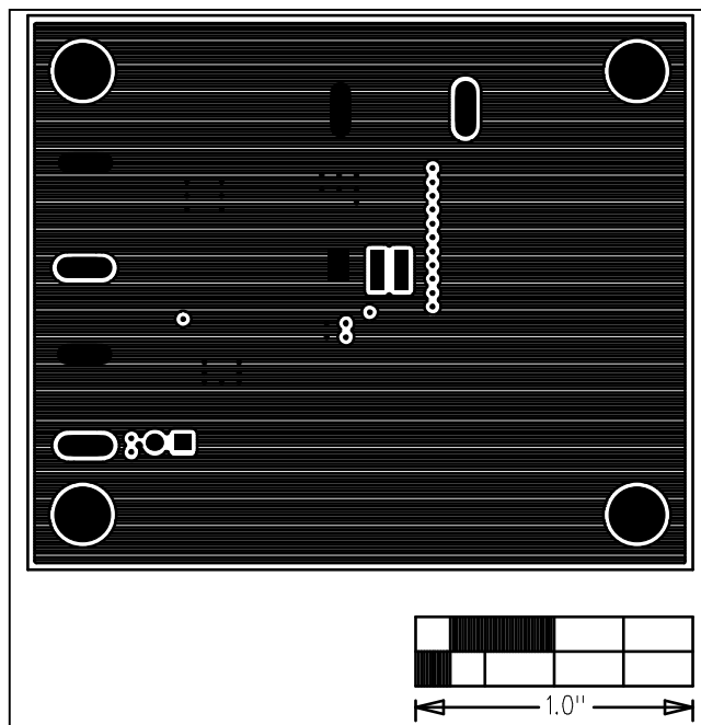
Figure 5. MAXM17515 EV Kit PCB Layout—PGND Layer 3
