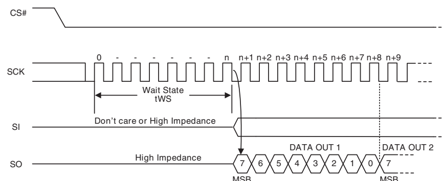
Figure 63. AutoBoot Sequence (CR1[1]=0)
