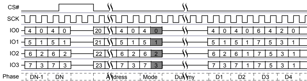
Figure 79. Continuous Quad I/O Read Command Sequence (3-Byte Address)
