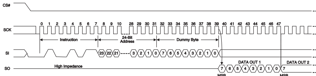
Figure 92. OTP Read Command Sequence
