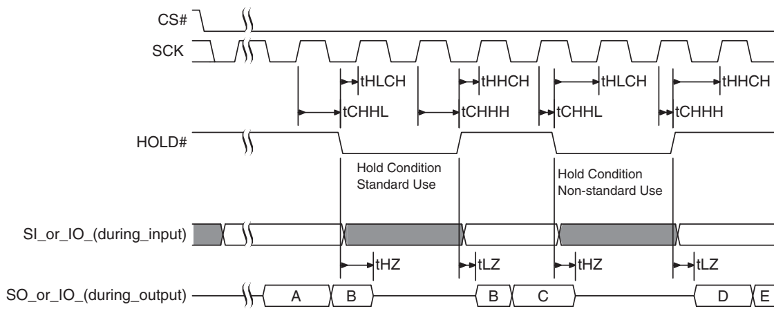
Figure 32. Hold Timing
