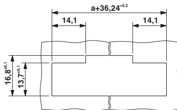
Dimensioned drawing
