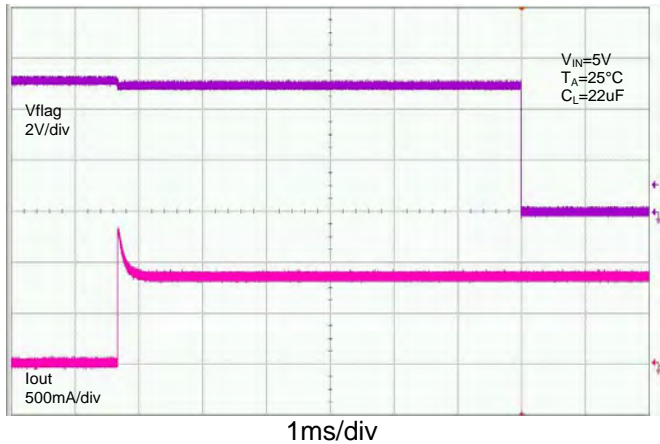
3 \Omega Load Connected to Enabled Device
