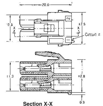
Section X-X
