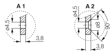
Barbed inserts
