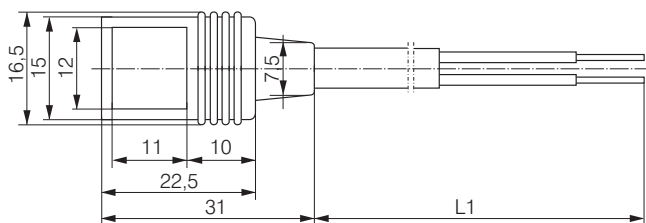
Connection cable
