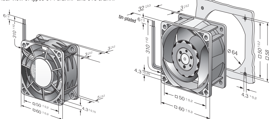
Rear view of types 614 J/2HHP and 618 J/2HHP
