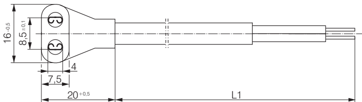
Angled plug (W)
