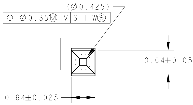
DETAIL C SCALE 20:1
