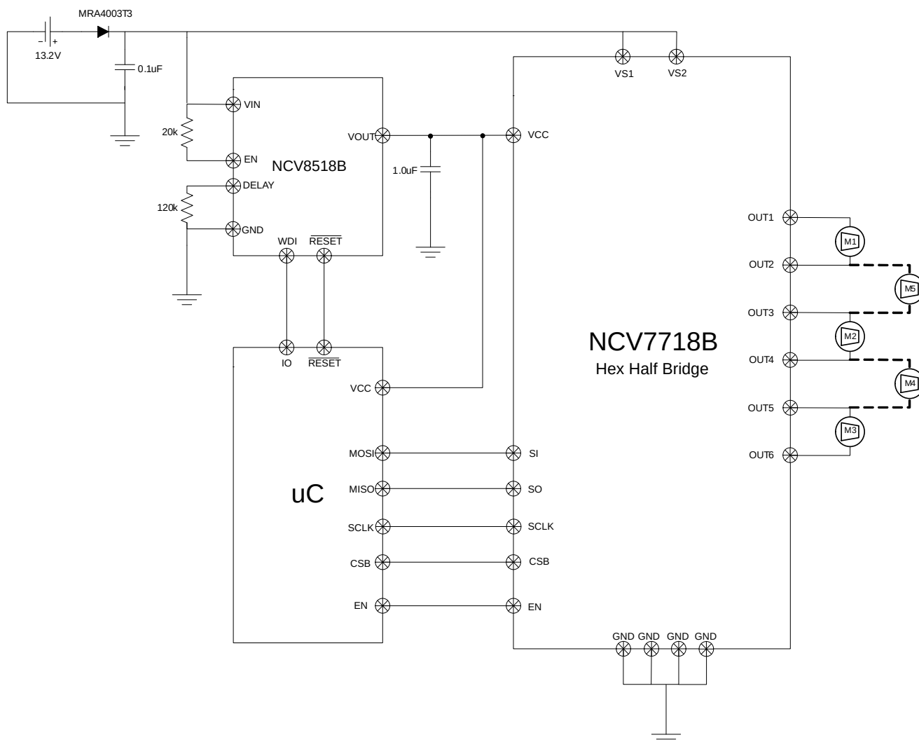
Figure 28. Application Drawing
