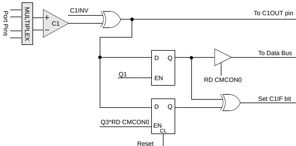
FIGURE 7-3: COMPARATOR C1 OUTPUT BLOCK DIAGRAM (PIC16F636/639)
