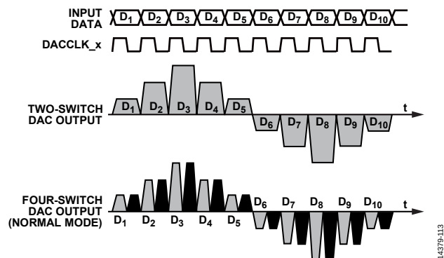
Figure 181. Two-Switch and Quad-Switch DAC Waveforms
