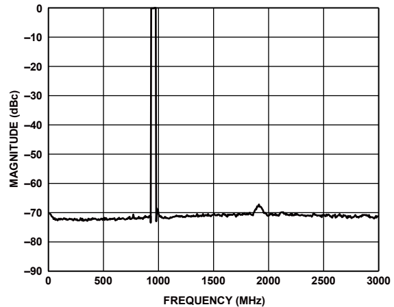
Figure 123. Eight Carriers at 950 MHz Output (Shuffle On)
