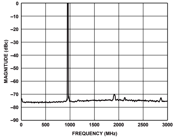
Figure 121. Four Carriers at 950 MHz Output (Shuffle On)
