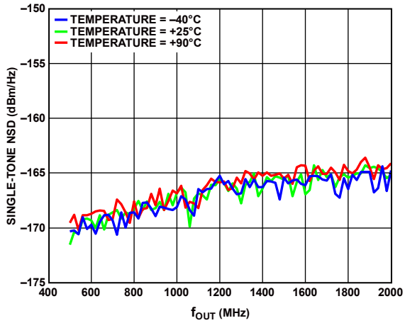
Figure 83. Single-Tone NSD Measured at 10% Offset from f_{OUT} vs. f_{OUT} over Temperature
