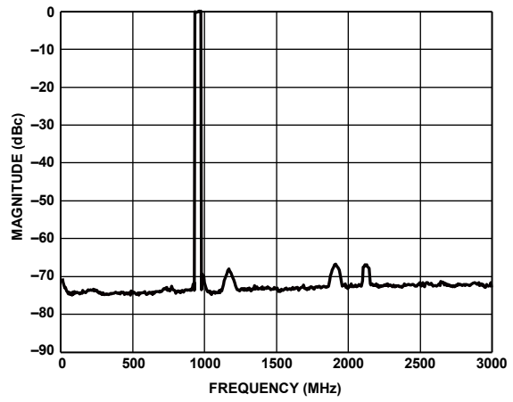
Figure 122. Eight Carriers at 950 MHz Output
