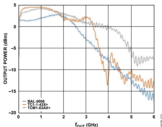
Figure 192. Measured DAC Output Response; f_{DAC} = 6 GSFS
