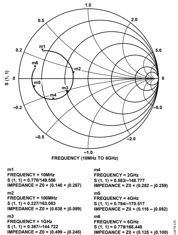
Figure 194. Simulated Smith Chart Showing the DAC Output Impedance ( Z_O = 100 \Omega )
