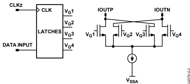
Figure 180. Quad-Switch Architecture
