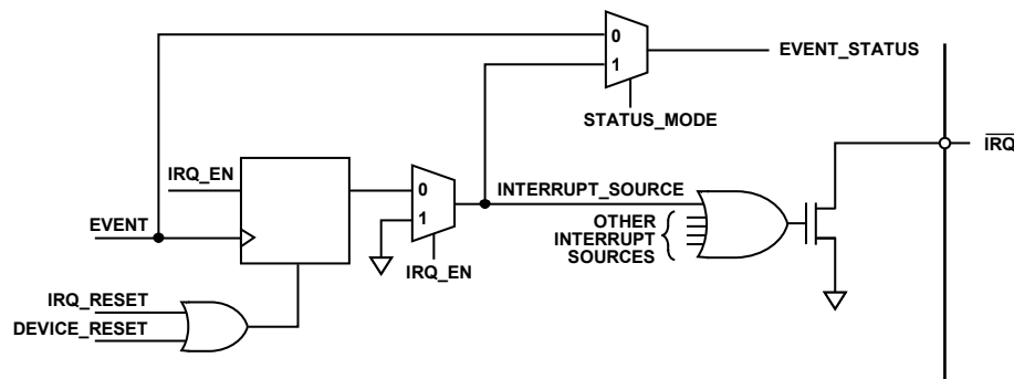
Figure 175. Simplified Schematic of \overline{IRQ} Circuitry
