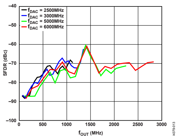
Figure 66. SFDR vs. f_{OUT} over f_{DAC}
