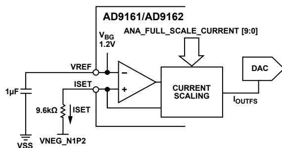
Figure 188. Voltage Reference Circuit
