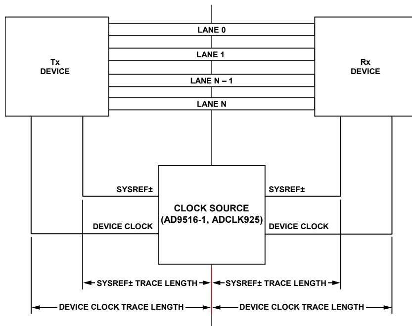
Figure 179. SYSREF \pm Signal and Device Clock Trace Length
