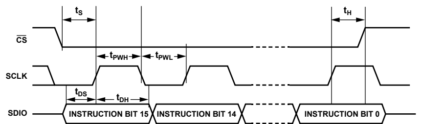
Figure 142. Timing Diagram for Serial Port Register Write
