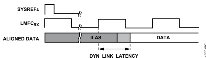
Figure 158. DYN_LINK_LATENCY_x Illustration
