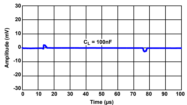
Figure 13. Line Transient with 100nF Load ( \Delta V_{IN} = \pm 500 mV)
