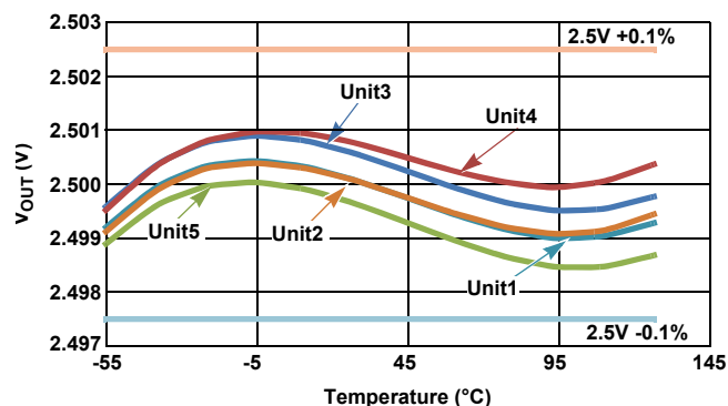
Figure 4. V_{OUT} vs Temperature, Five Units
