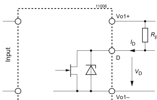
V_i, V_{o1} status D output, V_D V_i or V_{o1} < V_t low, L, V_D \leq 0.4 V at I_D = 2.5 mA V_i and V_{o1} > V_i + V_o high, H, I_D \leq 25 \mu A at V_D = 5.25 V
