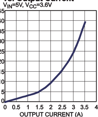
Case Temperature Rise vs. Output Current
