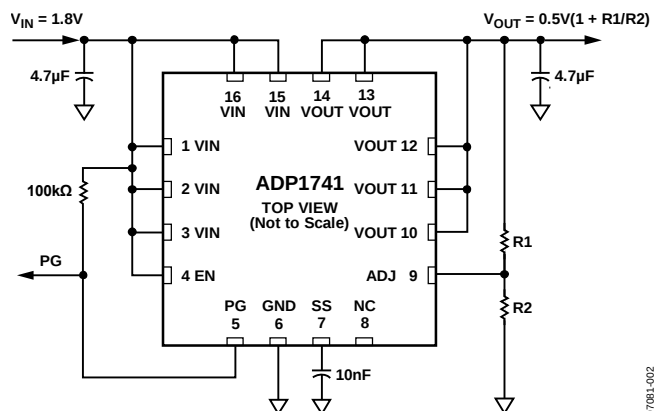
Figure 2. ADP1741 with Adjustable Output Voltage, 0.75 V to 3.3 V
