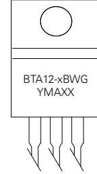
TO-220AB CASE 221A STYLE 12
