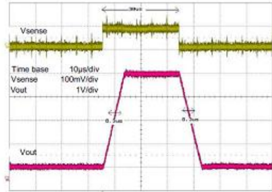
Figure 12: Step response
