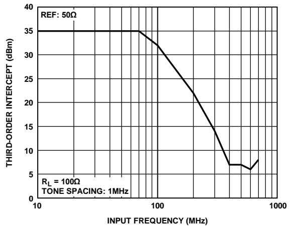
Figure 54. ADV3225 Output Third-Order Intercept, 100 \Omega Load
