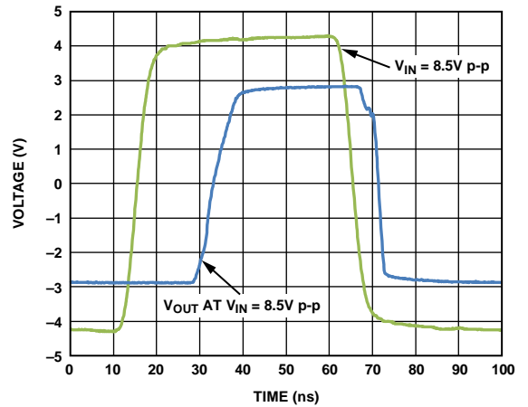
Figure 53. ADV3225 Overdrive Recovery
