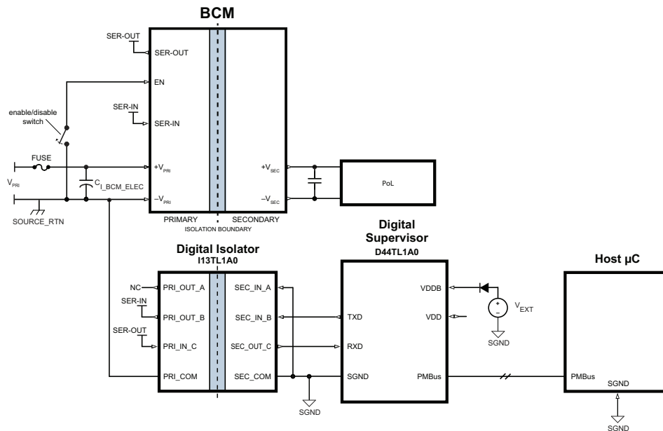
BCM6123xD1E5117y01 at point-of-load
