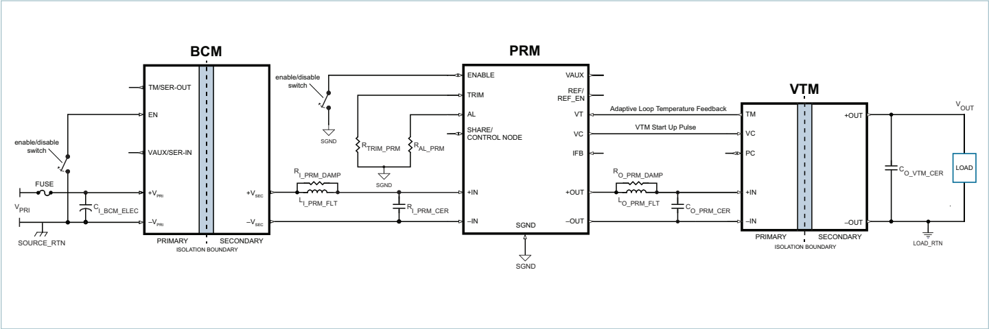
BCM6123xD1E5117yzz + PRM™ + VTM™, Adaptive-Loop configuration
