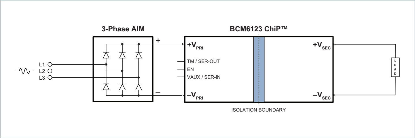
3-phase AC to point-of-load (3-phase AIM™ + BCM6123xD1E5117yzz)
