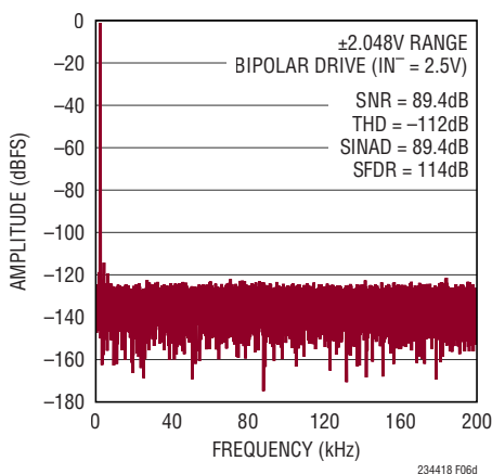
Figure 6d. IN^+ = -1\text{dBFS} 2kHz Bipolar Sine, IN^- = 2.5V , 32k Point FFT, f_{\text{SAMPL}} = 400\text{kps} . Circuit Shown in Figure 6a with LT6237 Amplifiers, R_{\text{FILT}} = 24.9\Omega , C_{\text{FILT}} = 1\text{nF}
