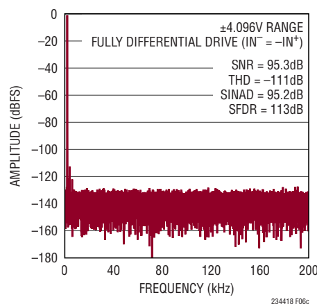
Figure 6c. IN^+/IN^- = -1\text{dBFS} 2kHz Fully Differential Sine, Common Mode = 2.5V, 32k Point FFT, f_{\text{SAMPL}} = 400\text{kps} . Circuit Shown in Figure 6a with LT6237 Amplifiers, R_{\text{FILT}} = 24.9\Omega , C_{\text{FILT}} = 1\text{nF}
