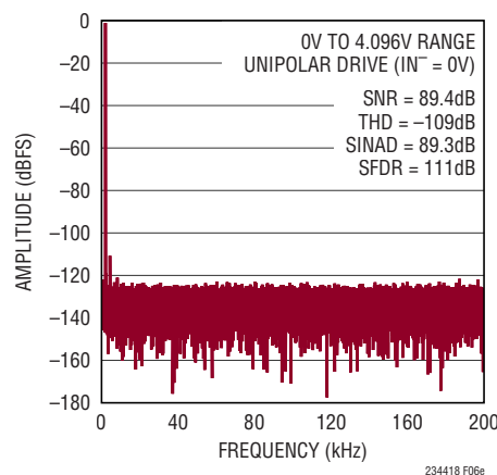
Figure 6e. IN^+ = -1\text{dBFS} 2kHz Unipolar Sine, IN^- = 0V , 32k Point FFT, f_{\text{SAMPL}} = 400\text{kps} . Circuit Shown in Figure 6a with LT6237 Amplifiers, R_{\text{FILT}} = 24.9\Omega , C_{\text{FILT}} = 1\text{nF}
