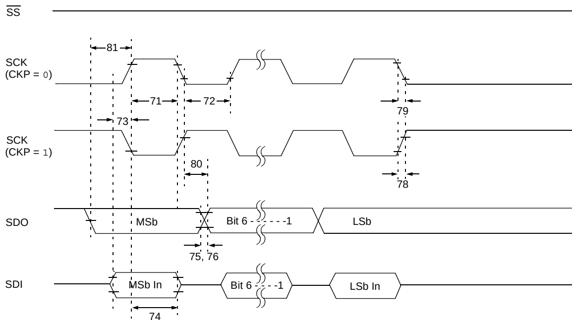
FIGURE 17-12: SPI MASTER MODE TIMING (CKE = 1, SMP = 1)
