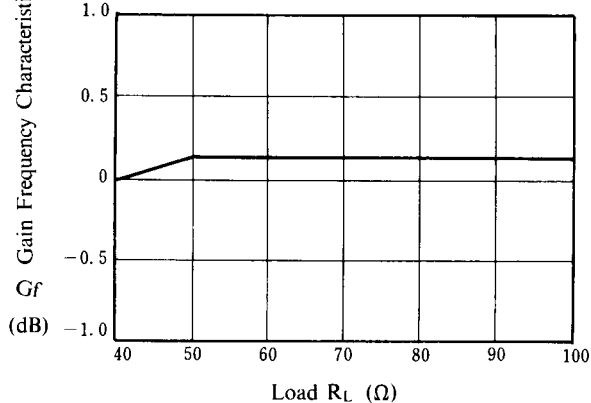
Gain Frequency Characteristics vs. R_L
