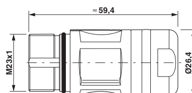
Dimensioned drawing
