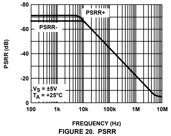
FIGURE 20. PSRR
