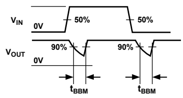
Figure 19. Break-Before-Make Time Delay, t_{BBM} (ADG619 Only)
