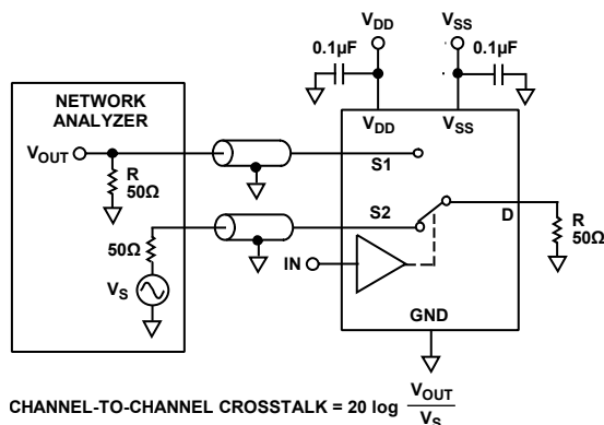
Figure 23. Channel-to-Channel Crosstalk
