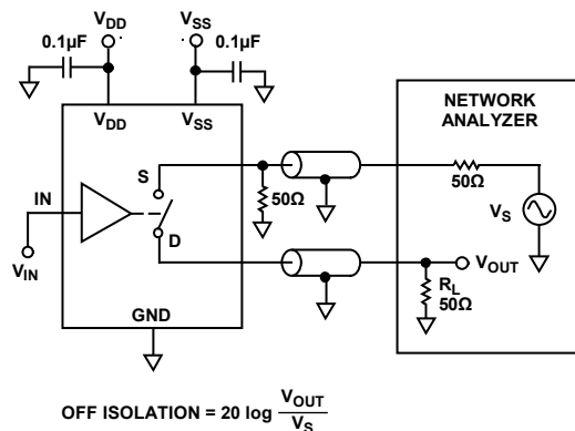
Figure 22. Off Isolation
