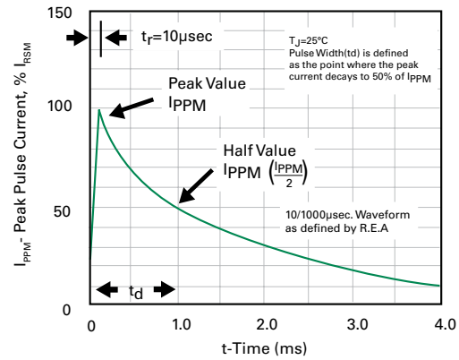
Figure 4 - Pulse Waveform
