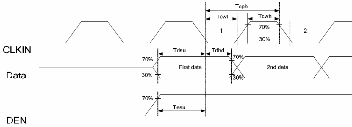
Figure 3: Pixel Timing
