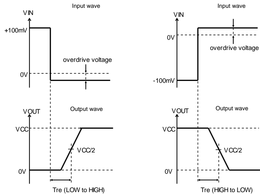
Figure 52. Response Time
