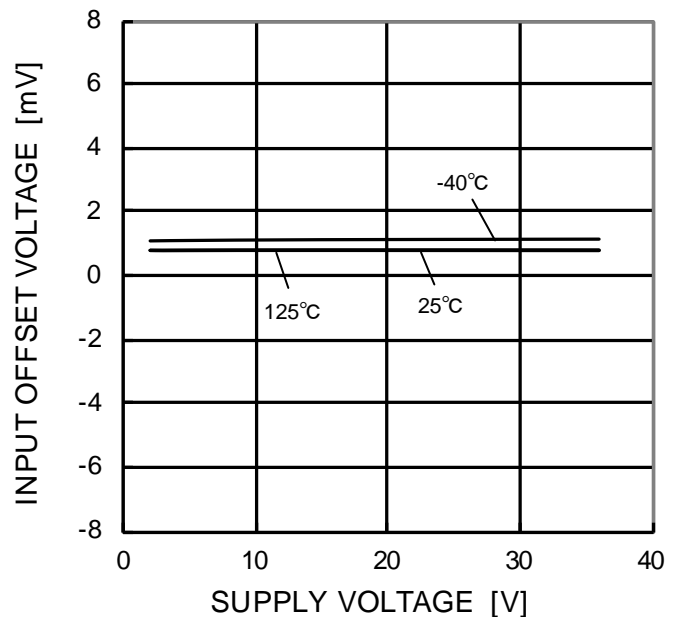
Figure 32. Input Offset Voltage – Supply Voltage
