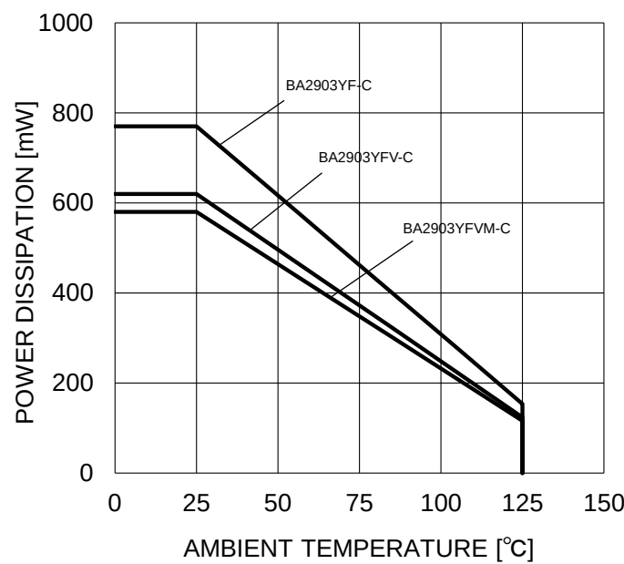
Figure 2. Derating Curve
