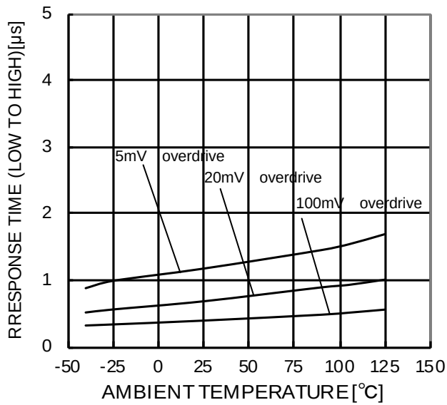
Figure 22. Response Time (Low to High) – Ambient Temperature (VCC=5V, VRL=5V, RL=5.1k \Omega )
