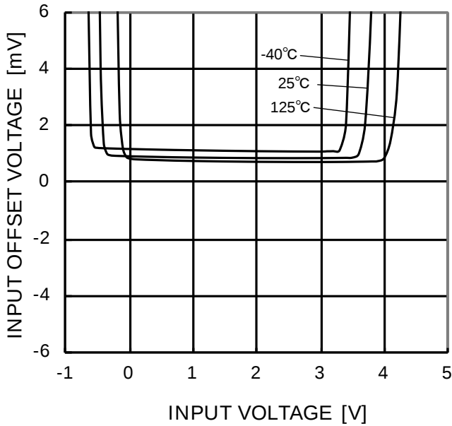
Figure 19. Input Offset Voltage – Input Voltage (VCC=5V)
