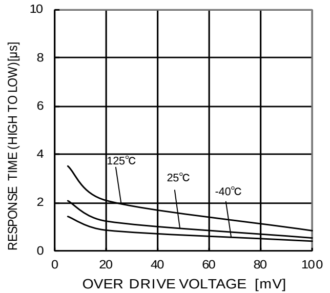
Figure 23. Response Time (High to Low) – Over Drive Voltage (VCC=5V, VRL=5V, RL=5.1k \Omega )
