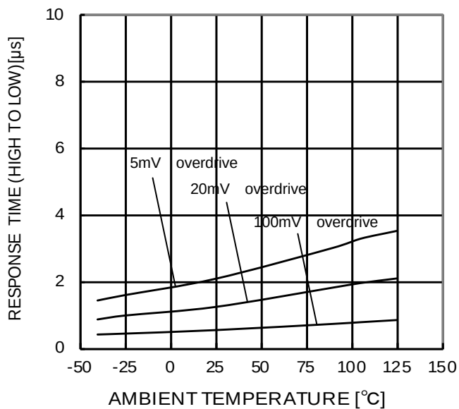
Figure 24. Response Time (High to Low) – Ambient Temperature (VCC=5V, VRL=5V, RL=5.1k \Omega )
