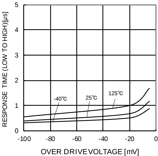
Figure 21. Response Time (Low to High) – Over Drive Voltage (VCC=5V, VRL=5V, RL=5.1kΩ)
