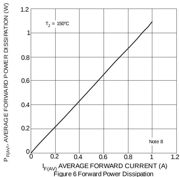
Figure 6 Forward Power Dissipation
