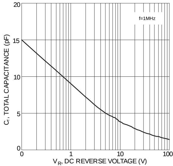
Figure 5 Total Capacitance
