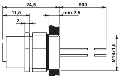
M12 flush-type plug, can be positioned
