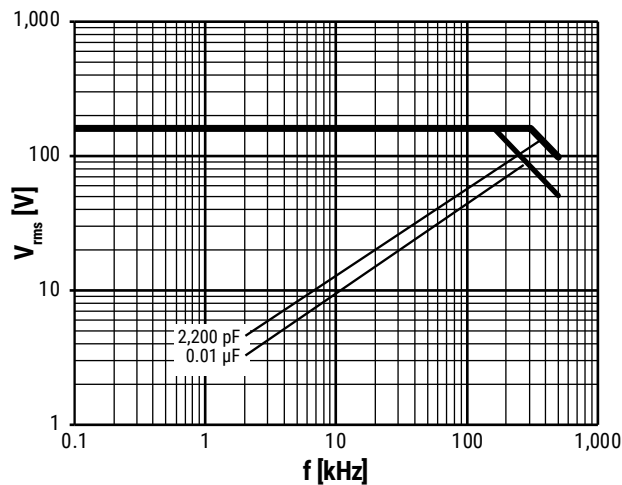
1,000 VDC/400 VAC
