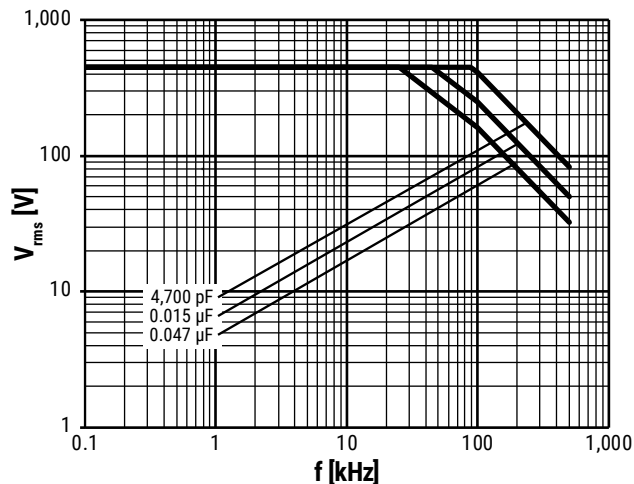
1,500 VDC/450 VAC
