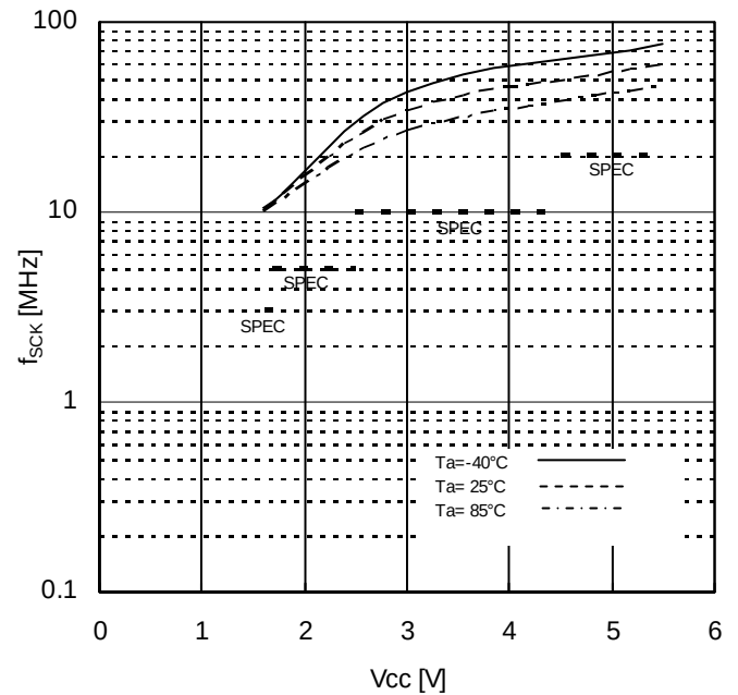
Figure 20. SCK Frequency vs Supply Voltage
