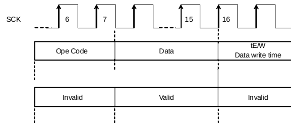
Figure 43. WPB valid timing (At inputting WRSR command)
