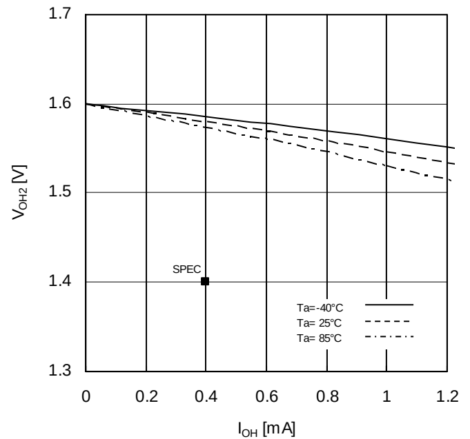
Figure 10. Output High Voltage2 vs Output Current (Vcc=1.6V)
