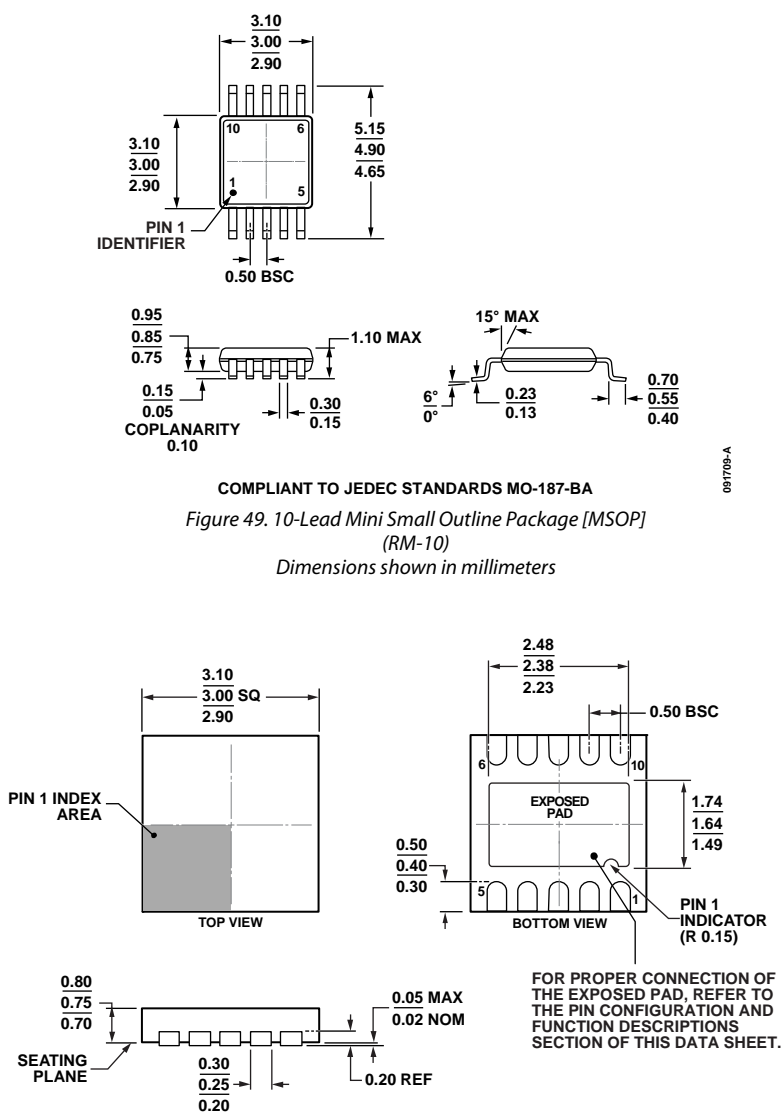
Figure 50. 10-Lead Lead Frame Chip Scale Package [QFN (LFCSP_WD)] 3 mm x 3 mm Body, Very Very Thin, Dual Lead (CP-10-9) Dimensions shown in millimeters
