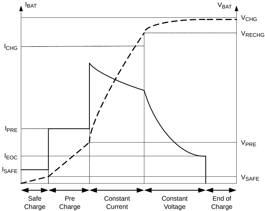
Figure 9. Typical Charging Profile of NCP1855 with Input Current Limit
