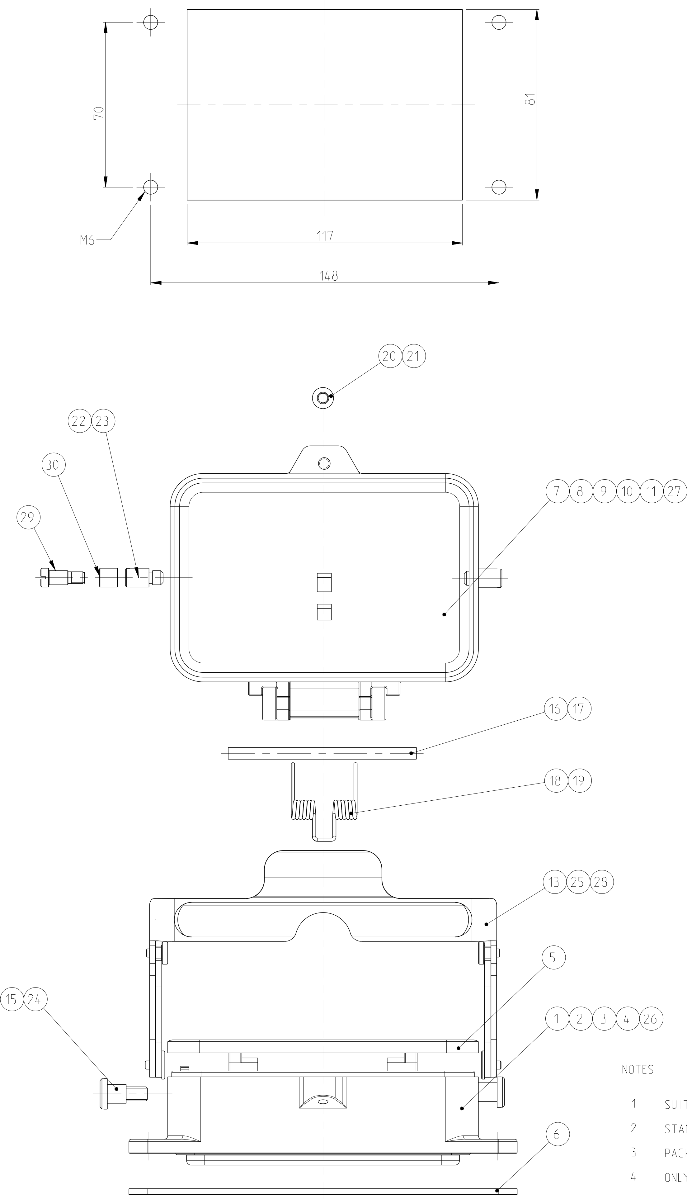
PANEL CUT-OUT
