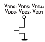
Figure 7. V_{DD6} to V_{DD1} Interface
