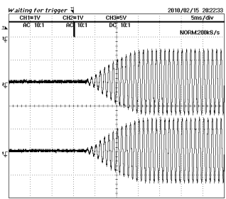
Fig.15 Advanced Switch 1
