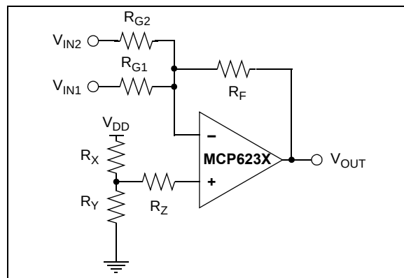
FIGURE 4-8: Summing Amplifier Circuit.
