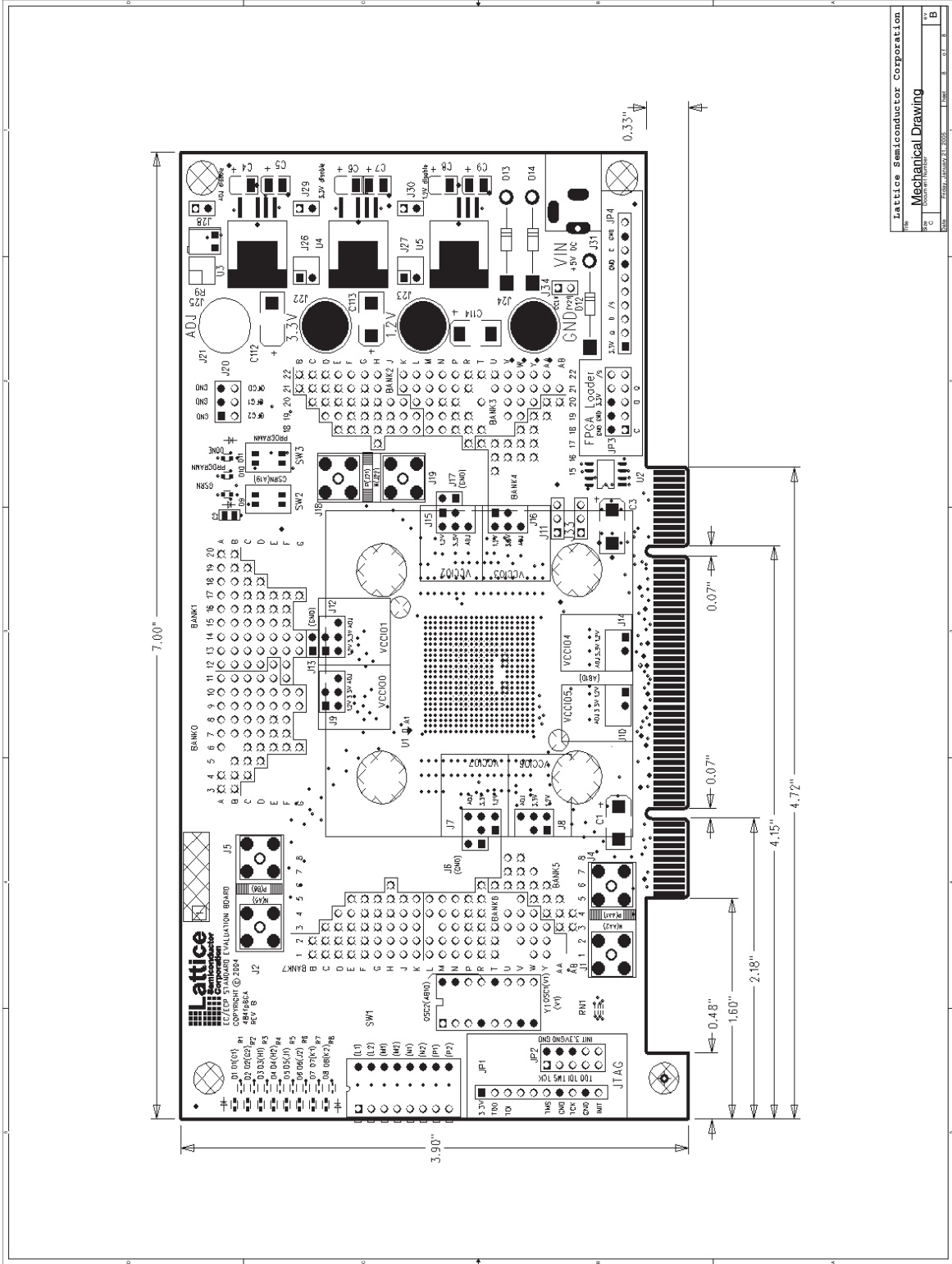
Figure 15. Mechanical Drawing
