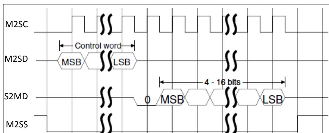
Figure 13. National Semiconductor Microwire Continuous Transfer
