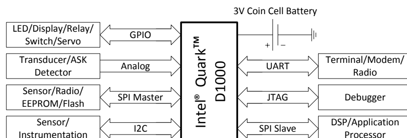
Figure 2. Example Application Demonstrating Usage of All MCU Interfaces
