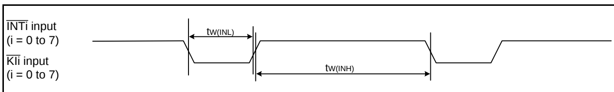
Figure 5.22 Input Timing of External Interrupt \overline{\text{INT}}i and Key Input Interrupt \overline{\text{KLI}}i
