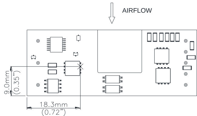
Figure 19: *Hot spot 1 temperature measured point. The allowed maximum hot spot 1 temperature is defined at 122 °C
